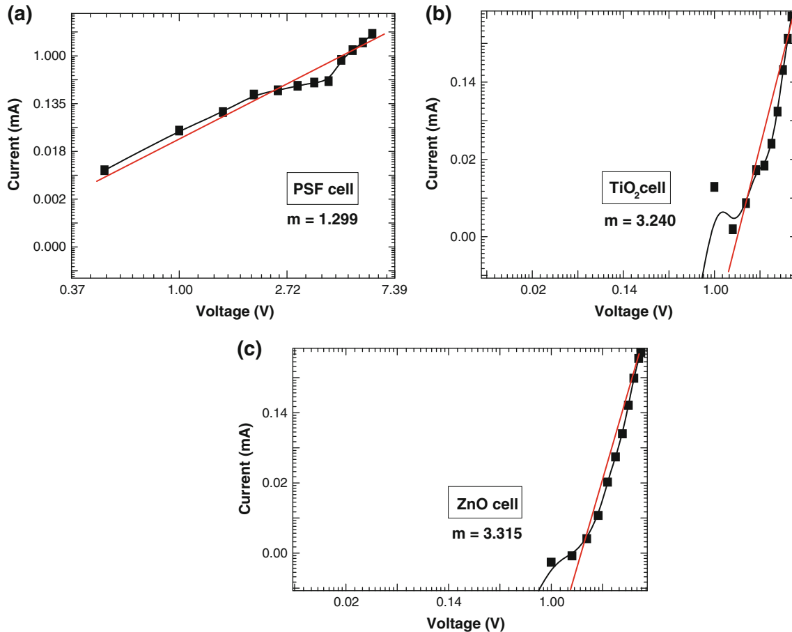
Fig. 5 ln I–ln V curves for (a) PSF cell, (b) TiO 2 cell, and (c) ZnO cell
